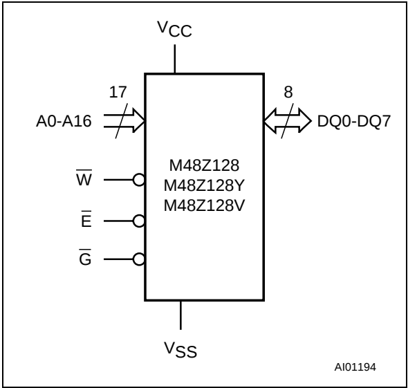
Figure 2. Logic Diagram
